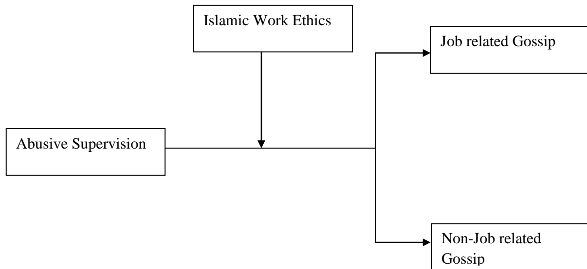
Figure-1: Theoretical Framework of Study
