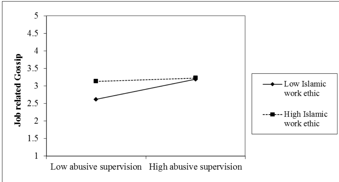
Figure-1: Moderation of IWE on Abusive supervision-Job related gossip relationship:
